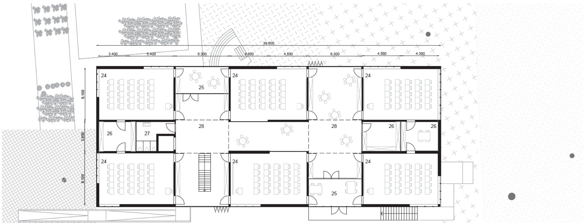
PLAN NIVEAU +1
